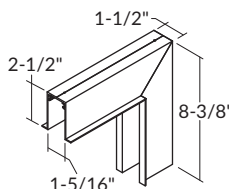
MP944-RFG Vertical Corner (Wall to Wall)
